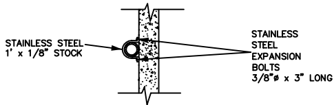
DETAIL A PLAN - STAINLESS STEEL STRAP
